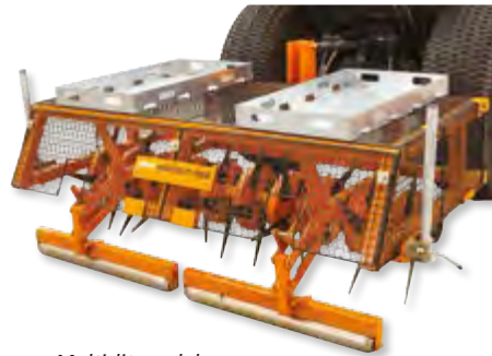
Multislit model
