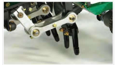
Reciprocating tines provide vertical coring action, punching straight in and out without tearing the turf, offering quality on par with golf courses.
